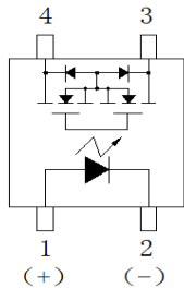
SMD4
