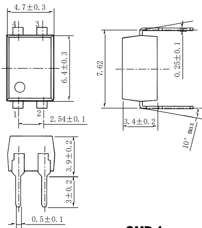
SMD4
